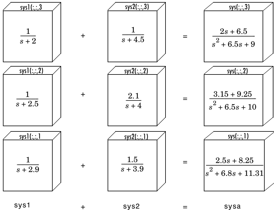
Figure 4-8: Addition of Two LTI Arrays
